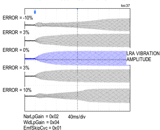
HAPTIC DRIVER LRA SELF-TUNING ERROR IN IniGss RESONANCE SETTING
