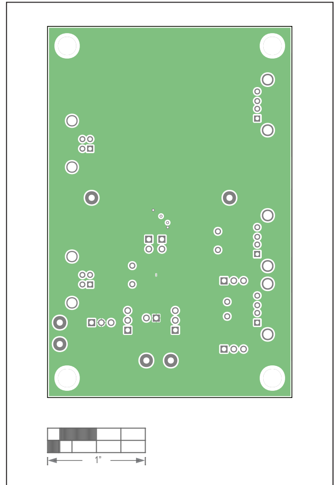
MAX20334 EV Kit—Layer 3 Power
