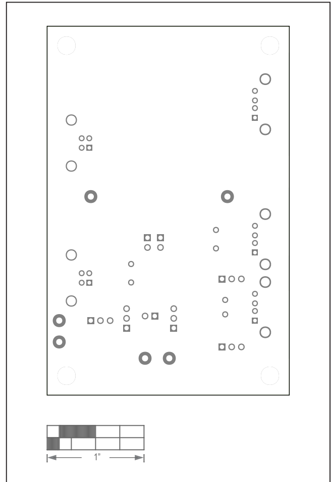
MAX20334 EV Kit—Bottom Silkscreen
