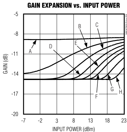
A = V_{GBP} = 0V E = V_{GBP} = 2.0V B = V_{GBP} = 0.5V F = V_{GBP} = 2.5V C = V_{GBP} = 1.0V G = V_{GBP} = 3.5V D = V_{GBP} = 1.5V H = V_{GBP} = 5.0V
