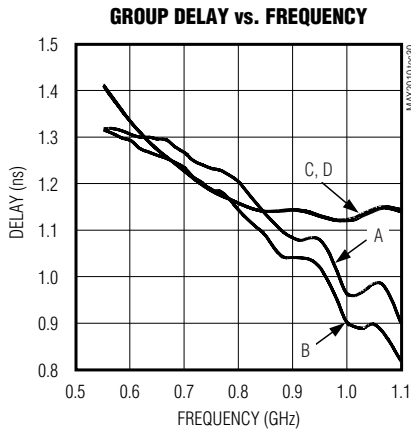
A = V_{GCS} = 0V , V_{GFS} = 0V C = V_{GCS} = 5V , V_{GFS} = 0V B = V_{GCS} = 0V , V_{GFS} = 5V D = V_{GCS} = 5V , V_{GFS} = 5V INTERCONNECTS DE-EMBEDDED
