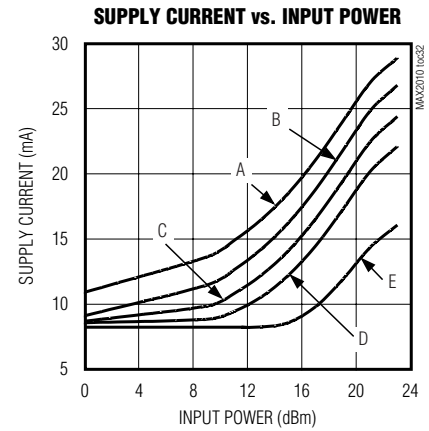
A = V_{GBP} = 0V D = V_{GBP} = 1.5V B = V_{GBP} = 0.5V E = V_{GBP} = 3.0V C = V_{GBP} = 1.0V
