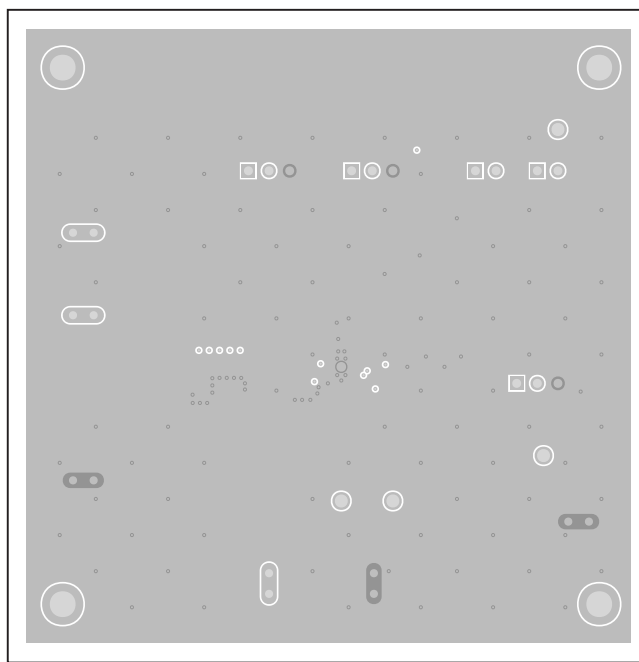
MAX20075/76 EV Kit PCB Layout—Internal Layer 3
