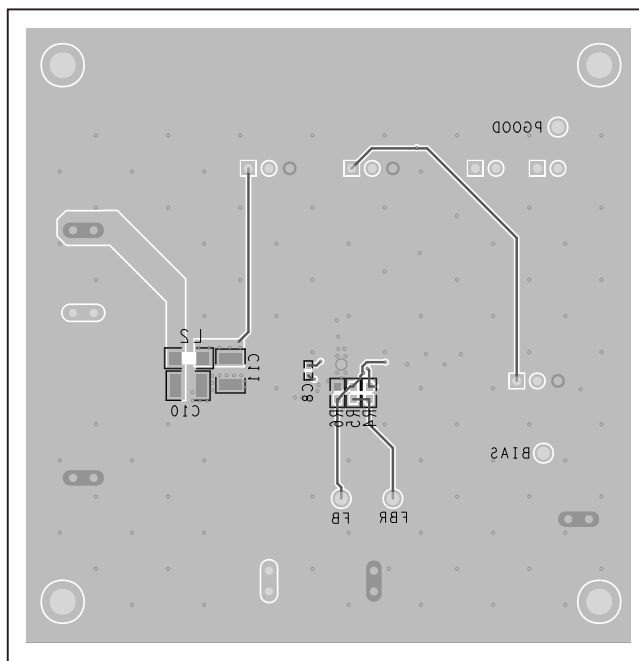
MAX20075/76 EV Kit Component Placement Guide—Bottom
