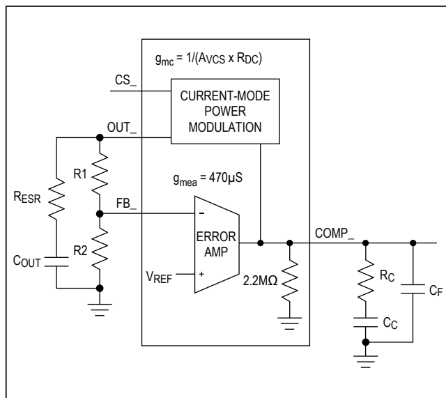
Figure 2. Compensation Network
