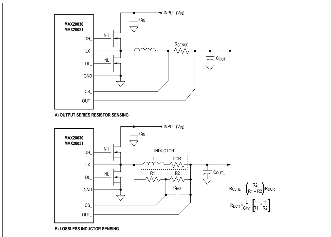
Figure 1. Current-Sense Configurations
