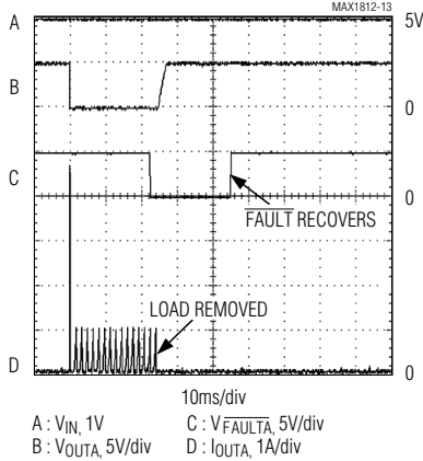
SHORT-CIRCUIT RESPONSE INTO 0\Omega
