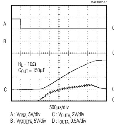
STARTUP TIME (TYPICAL USB APPLICATION)
