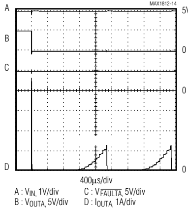
SHORT-CIRCUIT RESPONSE INTO 0\Omega LOAD (EXPANDED TIME SCALE)
