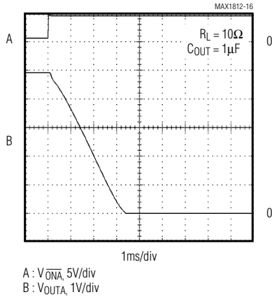
SWITCH TURN-OFF TIME
