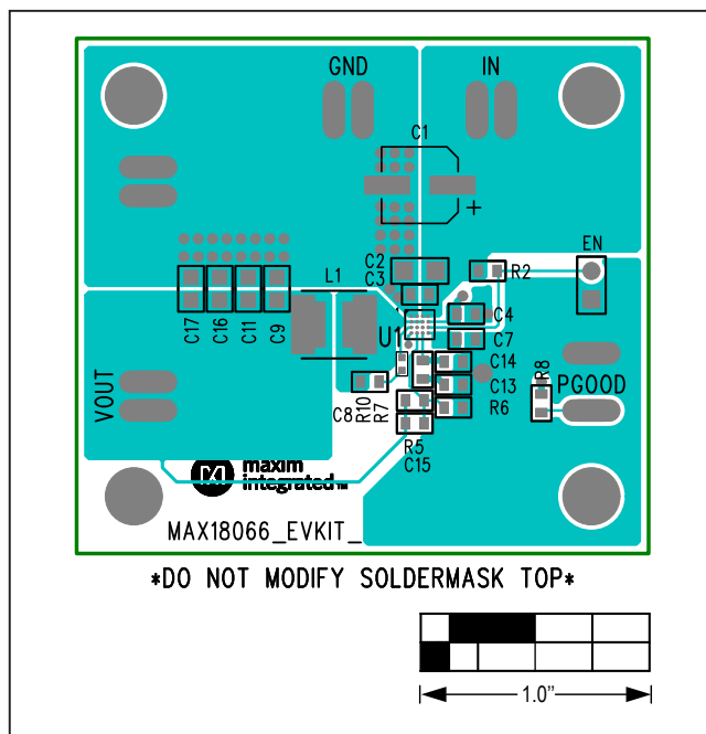
MAX18066 EV Component Placement Guide—Top View
