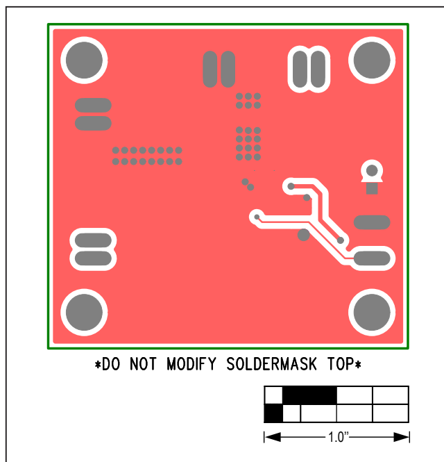
MAX18066 EV Component Placement Guide—Bottom View
