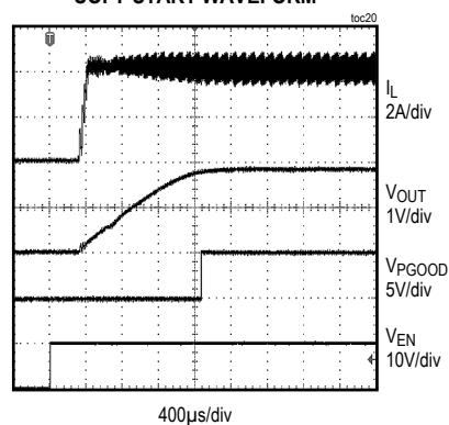
SOFT-START WAVEFORM
