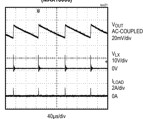
SKIP MODE WAVEFORM (MAX18066)
