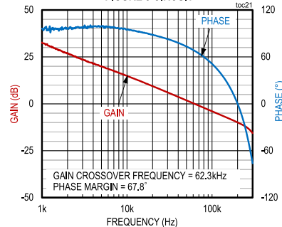
5V OUTPUT, BODE PLOT FIGURE 5 CIRCUIT
