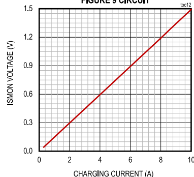
ISMON VOLTAGE vs. CHARGING CURRENT FIGURE 9 CIRCUIT
