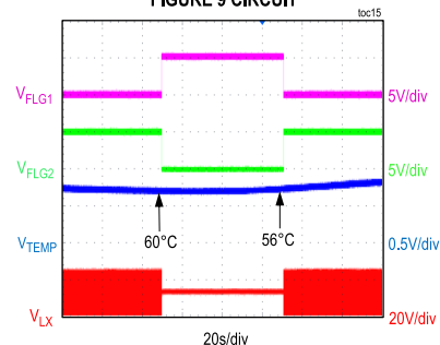
TEMP CHARGING DISABLE AND ENABLE FIGURE 9 CIRCUIT
