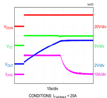
SUPERCAPACITOR CHARGING AT NO LOAD
