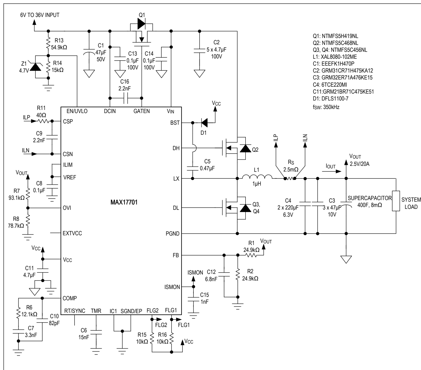
Figure 8. 2.5V/20A Supercapacitor Charger
