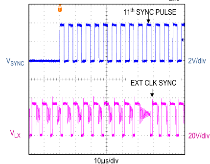
APPLICATION OF EXTERNAL CLOCK AT 180kHz, 5V OUTPUT, 0.15A LOAD FIGURE 11 CIRCUIT
