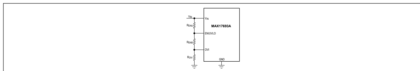
Figure 3. Programming EN/UVLO and OVI in MAX17693A
