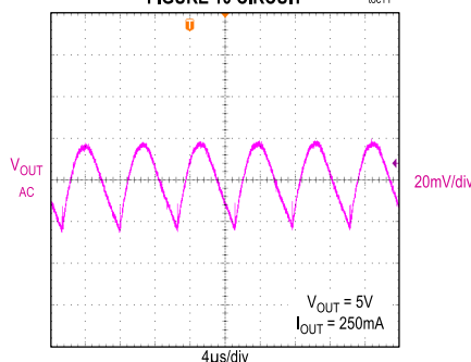
MAX17693A OUTPUT-VOLTAGE RIPPLE FIGURE 10 CIRCUIT
