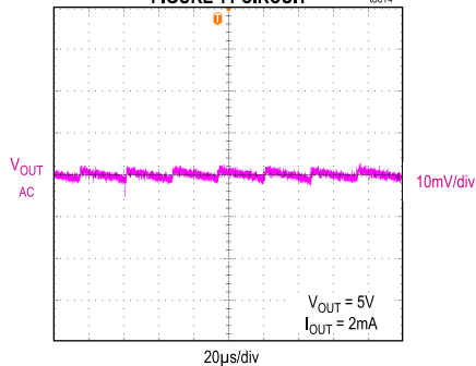
MAX17693B OUTPUT VOLTAGE RIPPLE FIGURE 11 CIRCUIT
