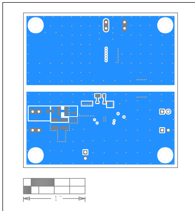
MAX17691A EV Kit PCB Layout—Bottom
