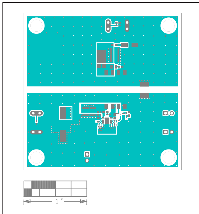
MAX17691A EV Kit PCB Layout—Top
