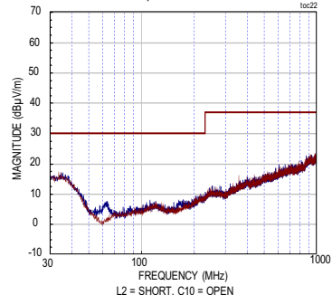
MAX17672C RADIATED EMISSIONS PLOT 5V OUTPUT, 150mA LOAD CURRENT
