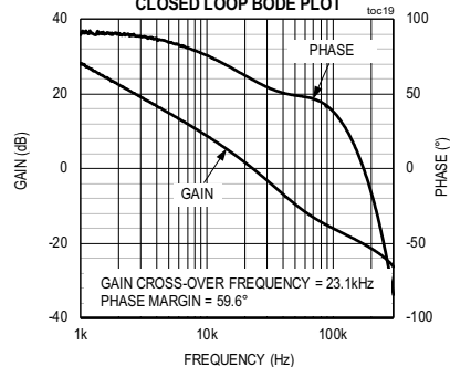
MAX17672C, 5V OUTPUT STEP-DOWN CONVERTER, CLOSED LOOP BODE PLOT
