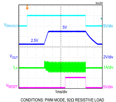
MAX17644C, V_{OUT3} = 5V SOFT-START/SHUTDOWN WITH PREBIAS VOLTAGE OF 2.5V
