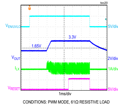
MAX17644A, V_{OUT1} = 3.3V SOFT-START/SHUTDOWN WITH PREBIAS VOLTAGE OF 1.65V
