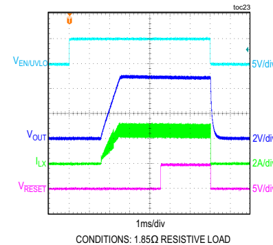
MAX17644C, V_{OUT3} = 5V SOFT-START/SHUTDOWN THROUGH EN/UVLO
