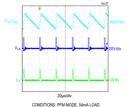
MAX17644A, V_{OUT1} = 3.3V STEADY STATE PERFORMANCE
