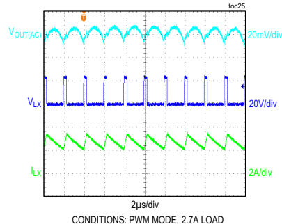
MAX17644A, V_{OUT1} = 3.3V STEADY STATE PERFORMANCE
