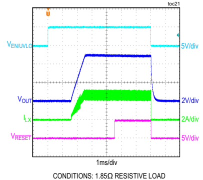
MAX17644B, V_{OUT2} = 5V SOFT-START/SHUTDOWN THROUGH EN/UVLO
