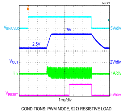
MAX17644B, V_{OUT2} = 5V SOFT-START/SHUTDOWN WITH PREBIAS VOLTAGE OF 2.5V
