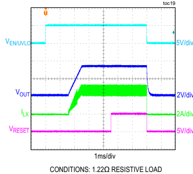
MAX17644A, V_{OUT1} = 3.3V SOFT-START/SHUTDOWN THROUGH EN/UVLO
