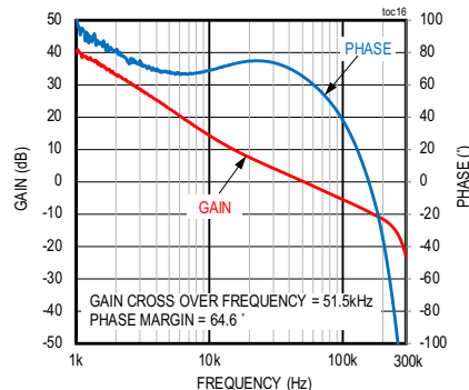
BODE PLOT
