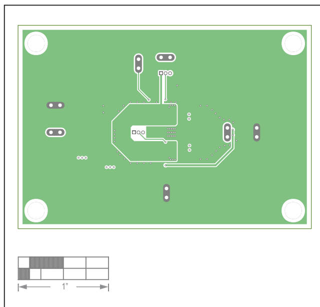
MAX17634C EV Kit—Layer3 GND
