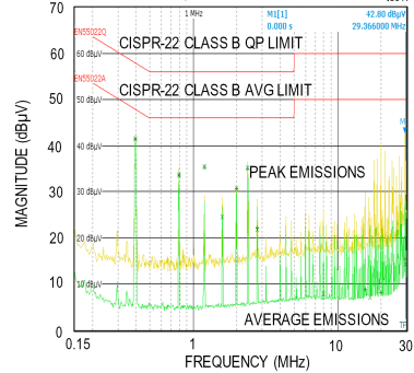
CONDUCTED EMISSIONS PLOT 5V OUTPUT, 4.25A LOAD CURRENT
