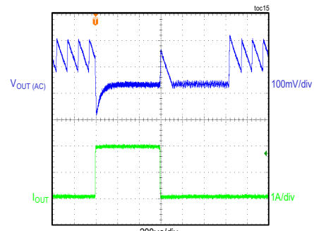
LOAD TRANSIENT BETWEEN 0.05A AND 2A
