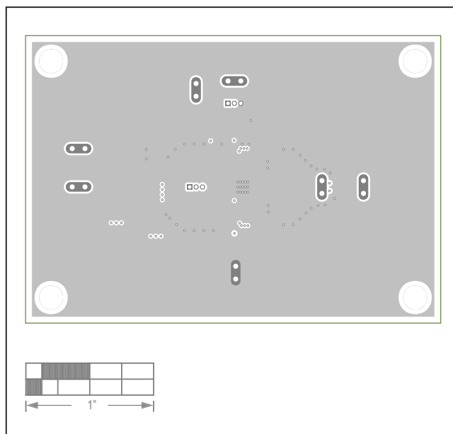
MAX17634C EV Kit—Layer2 GND
