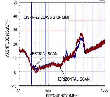
RADIATED EMISSIONS PLOT 5V OUTPUT, 4.25A LOAD CURRENT
