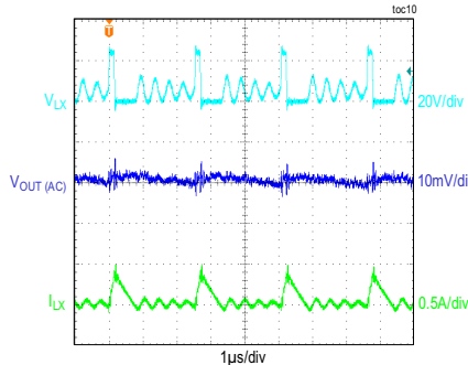
STEADY-STATE PERFORMANCE
