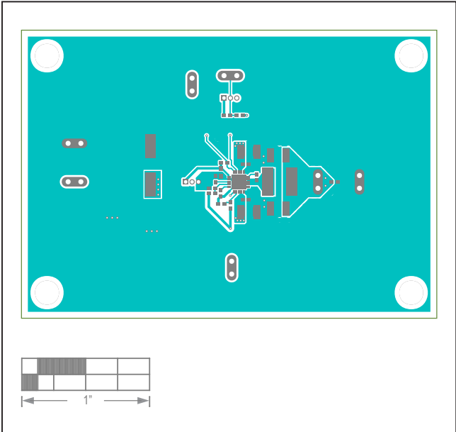
MAX17634B EV Kit—Top
