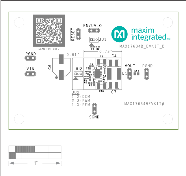
MAX17634B EV Kit—Top Silkscreen
