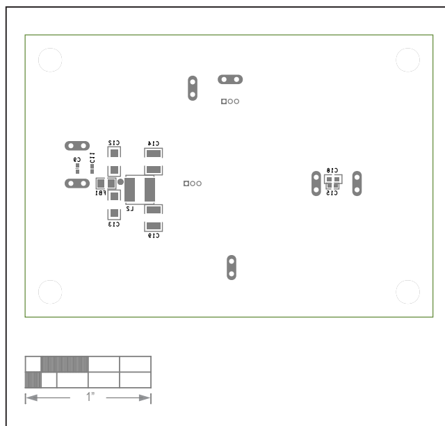
MAX17634B EV Kit—Bottom Silkscreen
