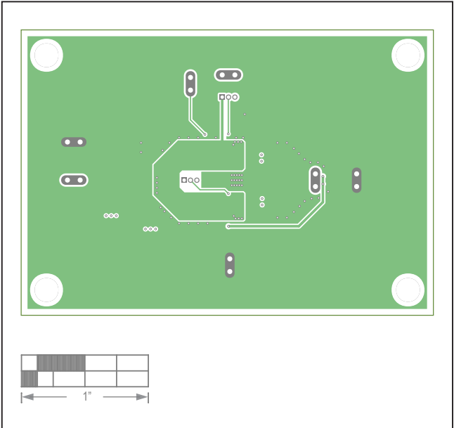
MAX17634B EV Kit—Layer3 GND
