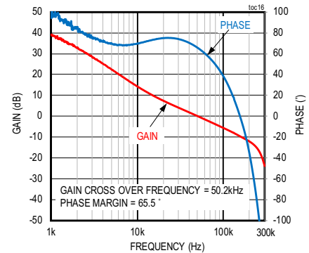
BODE PLOT
