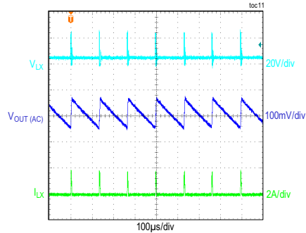
STEADY-STATE PERFORMANCE
