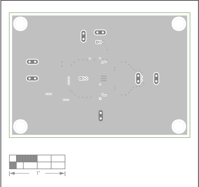
MAX17634B EV Kit—Layer2 GND
