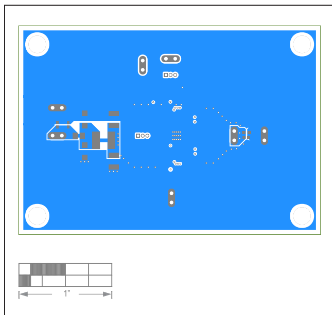
MAX17634B EV Kit—Bottom
