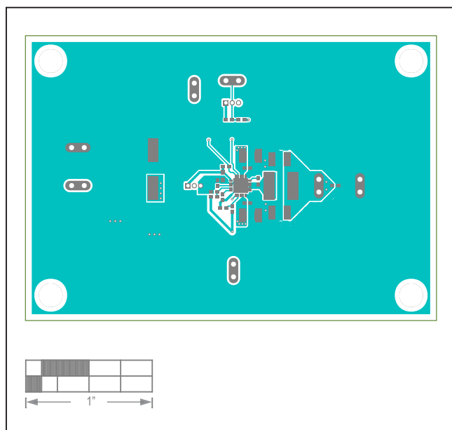
MAX17634A EV Kit—Top
