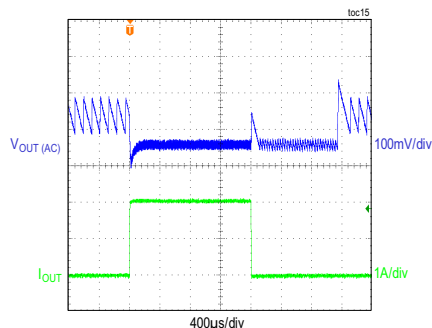
LOAD TRANSIENT BETWEEN 0.05A AND 2A
