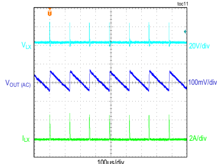
STEADY-STATE PERFORMANCE
