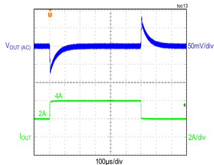
LOAD TRANSIENT BETWEEN 2A AND 4A
