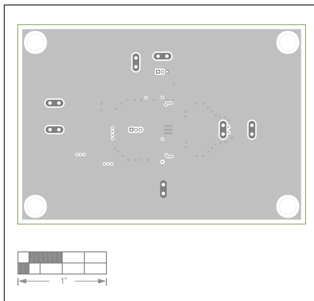
MAX17634A EV Kit—Layer2 GND
