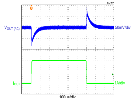
LOAD TRANSIENT BETWEEN 0A AND 2A
