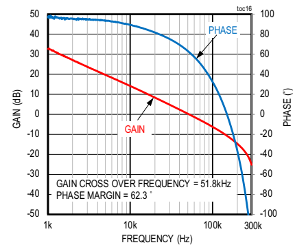
BODE PLOT
