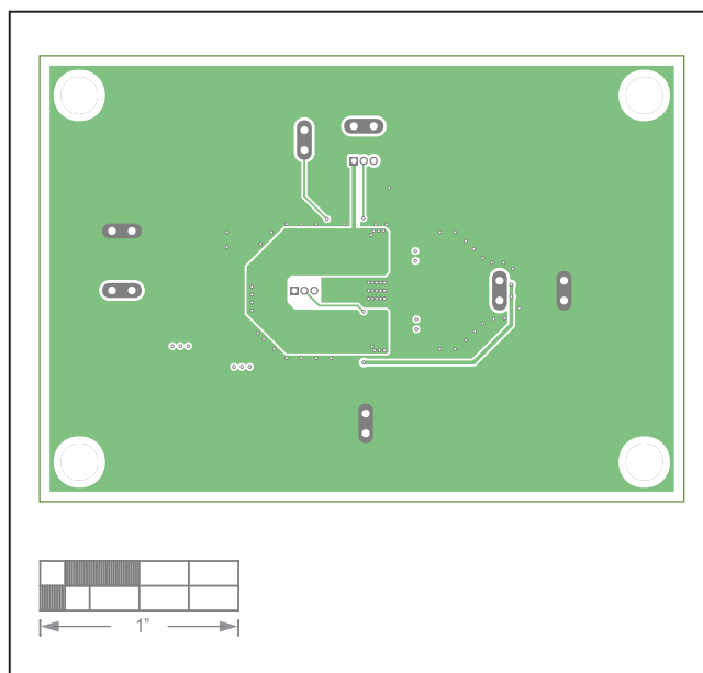
MAX17634A EV Kit—Layer3 GND
