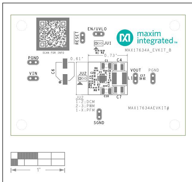
MAX17634A EV Kit—Top Silkscreen
