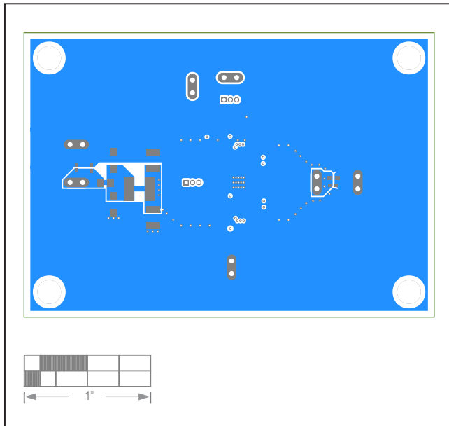
MAX17634A EV Kit—Bottom
