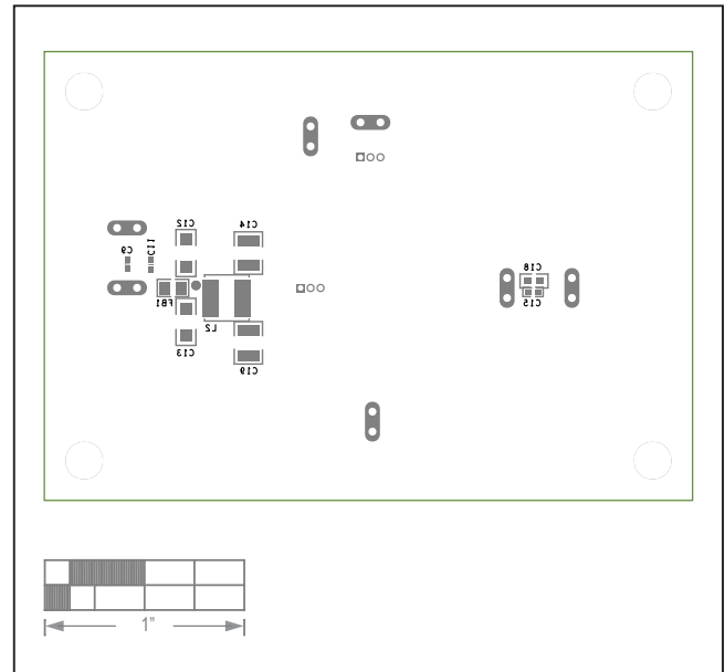
MAX17634A EV Kit—Bottom Silkscreen
