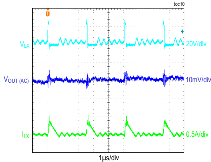
STEADY-STATE PERFORMANCE
