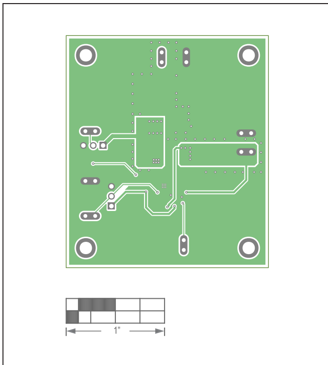
MAX17631BEVKIT# EV Kit—Layer 3
