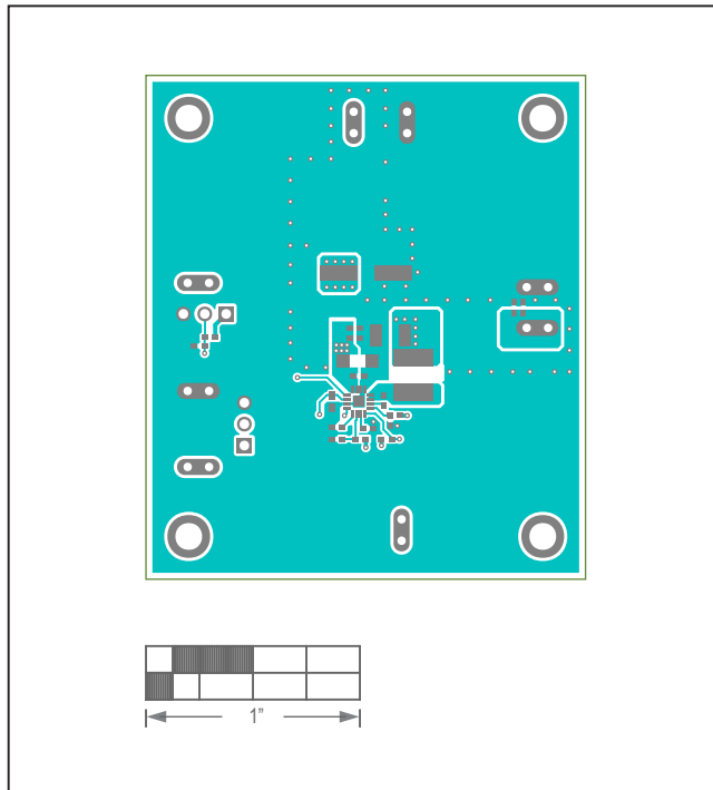
MAX17631BEVKIT# EV Kit—Top Layer
