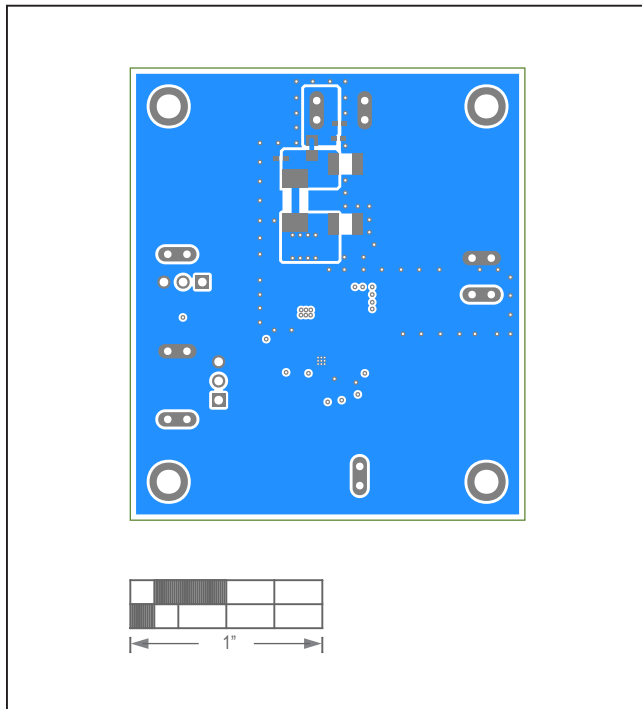
MAX17631BEVKIT# EV Kit—Bottom Layer
