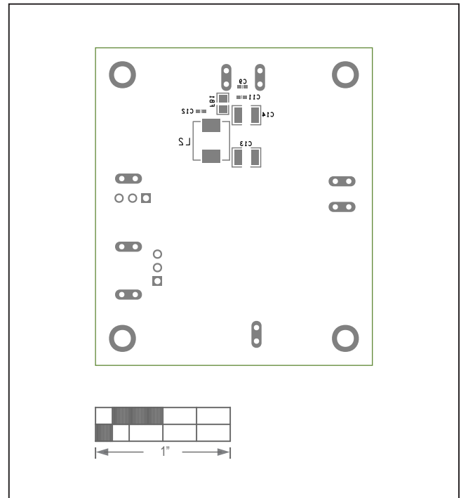
MAX17631BEVKIT# EV Kit—Bottom Silkscreen
