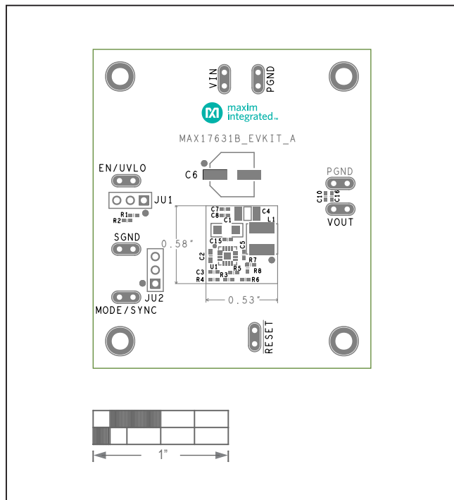
MAX17631BEVKIT# EV Kit—Top Silkscreen
