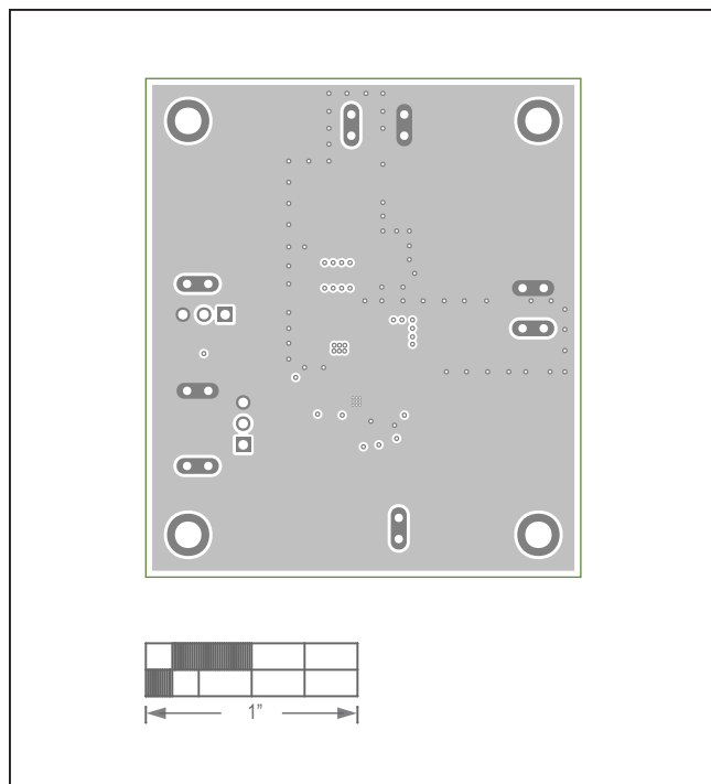
MAX17631BEVKIT# EV Kit—Layer 2
