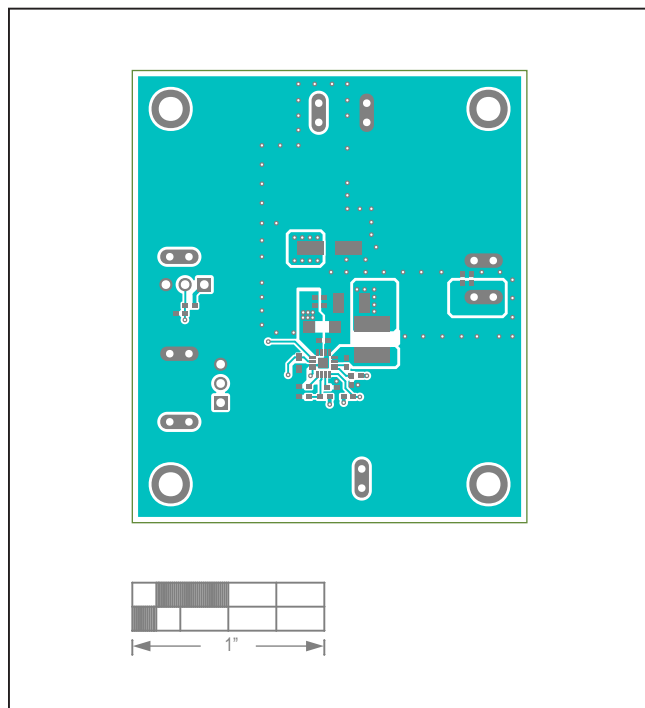
MAX17630C5EVKIT# EV Kit—Top Layer
