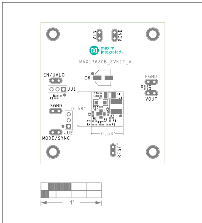
MAX17630BEVKIT# EV Kit—Top Silkscreen
