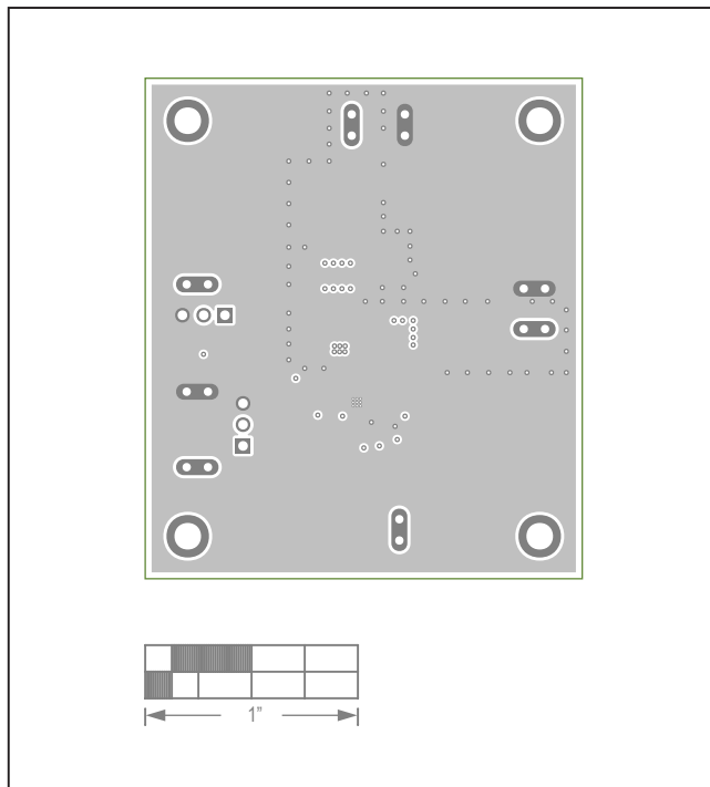
MAX17630BEVKIT# EV Kit—Layer 2
