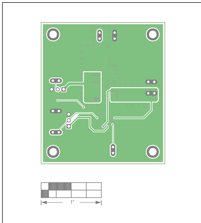
MAX17630BEVKIT# EV Kit—Layer 3
