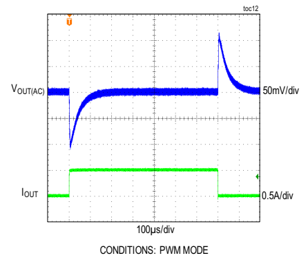
LOAD TRANSIENT RESPONSE BETWEEN 0A AND 0.5A
