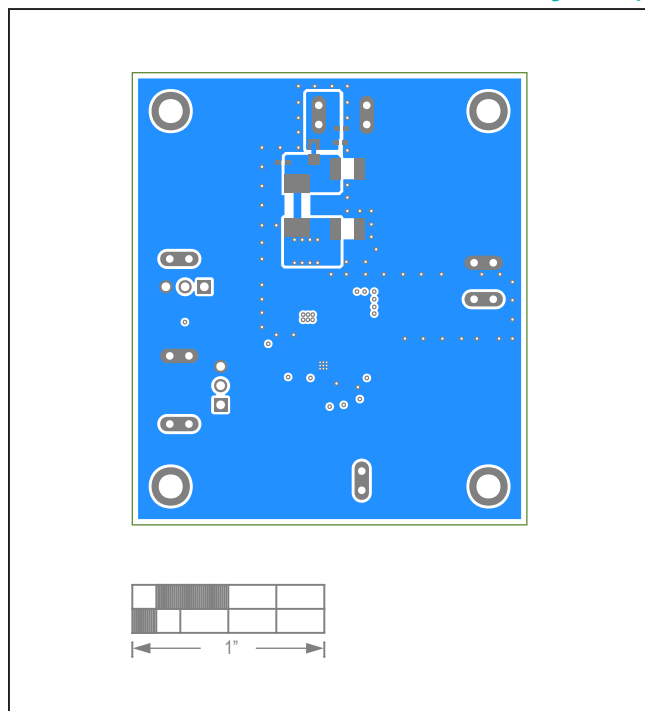
MAX17630BEVKIT# EV Kit—Bottom Layer
