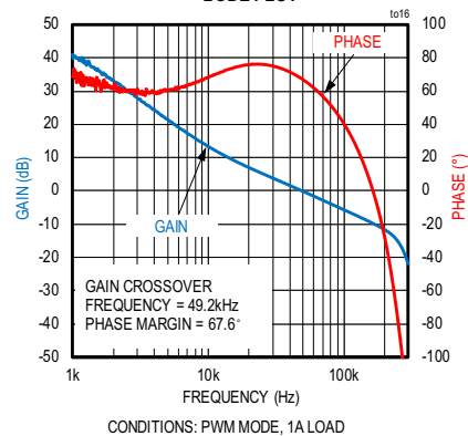
BODE PLOT
