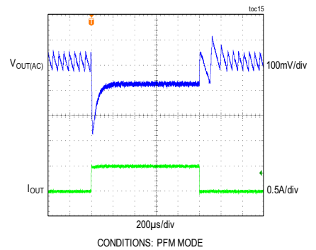
LOAD TRANSIENT RESPONSE BETWEEN 20mA AND 0.5A
