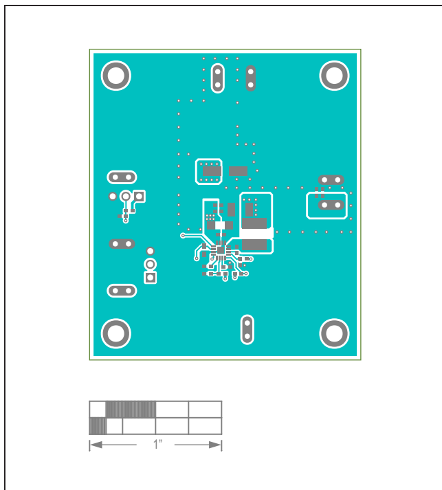
MAX17630BEVKIT# EV Kit—Top Layer
