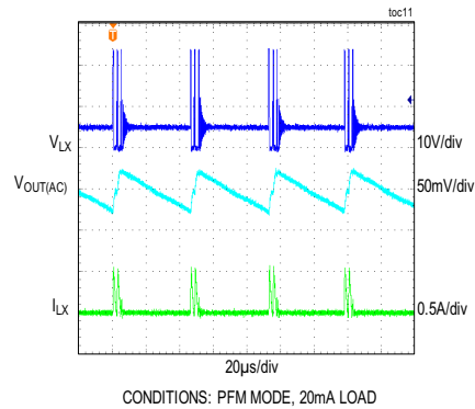
STEADY-STATE PERFORMANCE
