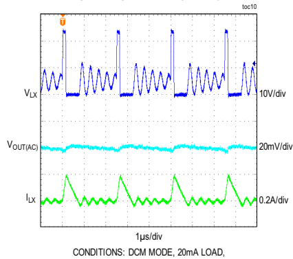
STEADY-STATE PERFORMANCE
