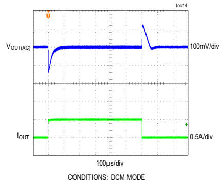
LOAD TRANSIENT RESPONSE BETWEEN 20mA AND 0.5A
