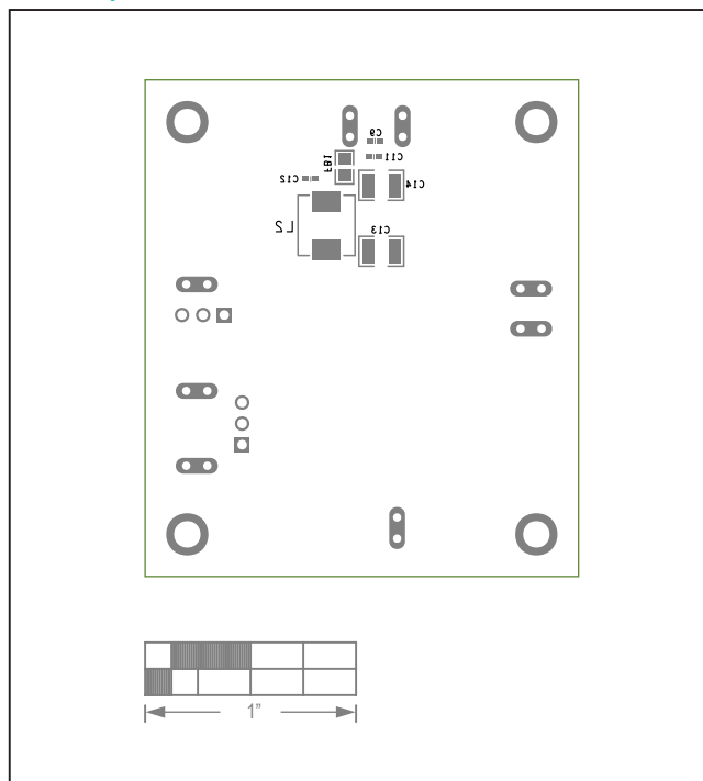
MAX17630BEVKIT# EV Kit—Bottom Silkscreen
