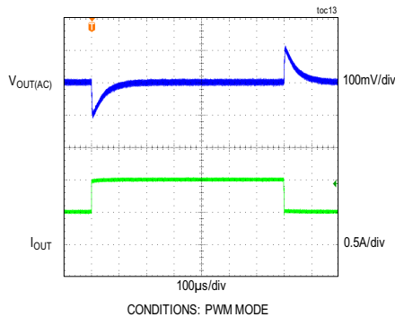
LOAD TRANSIENT RESPONSE BETWEEN 0.5A AND 1A
