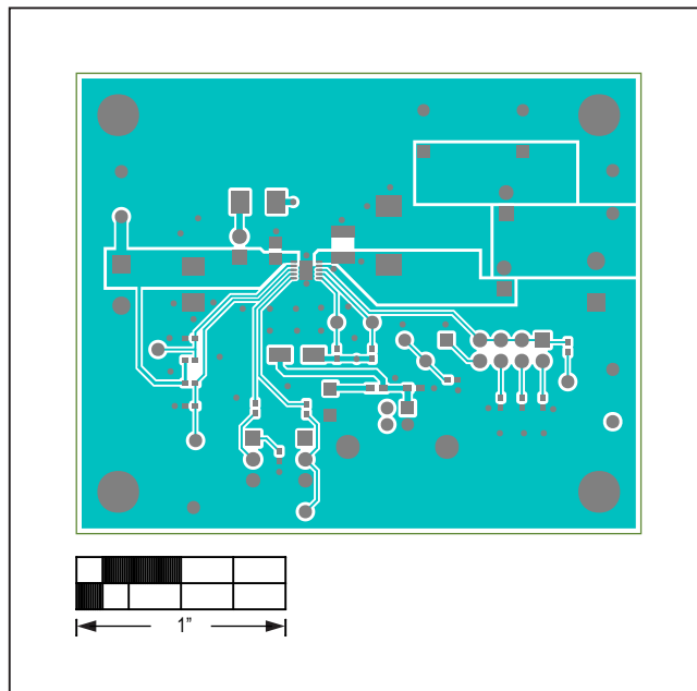
MAX17612B EV Kit PCB Layout—Top Layer
