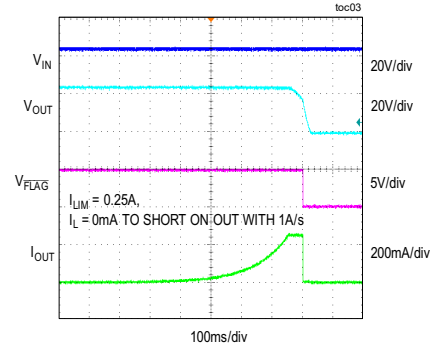
CURRENT-LIMIT RESPONSE
