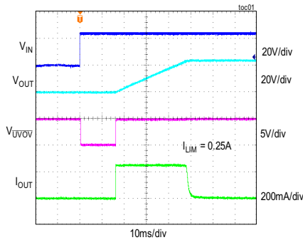
POWER-UP RESPONSE WITH 330 \mu F CAPACITOR AT NO LOAD
