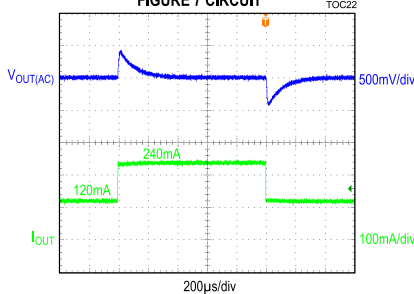
MAX17579/MAX17580, -15V OUTPUT, LOAD TRANSIENT BETWEEN 120mA AND 240mA, FIGURE 7 CIRCUIT
