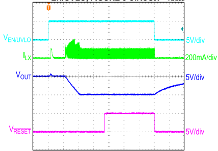
MAX17580, -5V OUTPUT, SOFT-START AND SHUTDOWN THROUGH EN/UVLO, FIGURE 5 CIRCUIT
