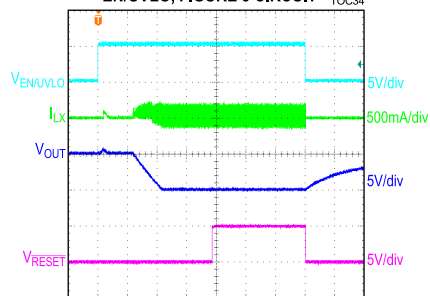
MAX17579, -5V OUTPUT, SOFT-START AND SHUTDOWN THROUGH EN/UVLO, FIGURE 5 CIRCUIT
