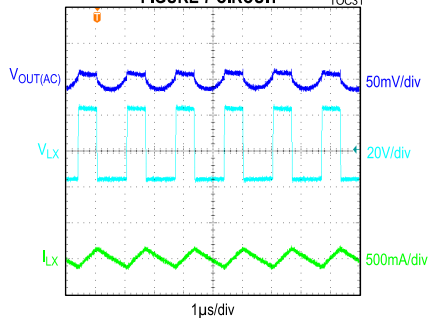
MAX17579, -15V OUTPUT, STEADY-STATE, FIGURE 7 CIRCUIT
