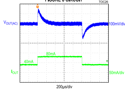
MAX17579, -15V OUTPUT, LOAD TRANSIENT BETWEEN 40mA AND 80mA, FIGURE 8 CIRCUIT
