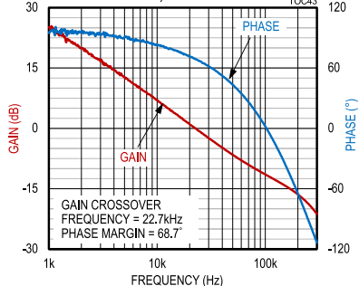
MAX17579/MAX17580, -15V OUTPUT, BODE PLOT, FIGURE 7 CIRCUIT
