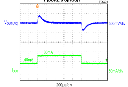
MAX17579, -15V OUTPUT, LOAD TRANSIENT BETWEEN 40mA AND 80mA, FIGURE 8 CIRCUIT
