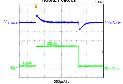
MAX17580, -15V OUTPUT, LOAD TRANSIENT BETWEEN 12mA AND 120mA, FIGURE 7 CIRCUIT
