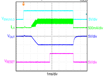
MAX17579/MAX17580, -5V OUTPUT, SOFT-START AND SHUTDOWN THROUGH EN/UVLO, FIGURE 5 CIRCUIT
