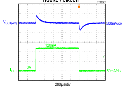
MAX17579, -15V OUTPUT, LOAD TRANSIENT BETWEEN 0A AND 120mA, FIGURE 7 CIRCUIT
