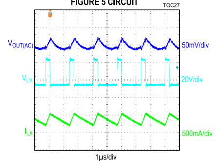
MAX17579/MAX17580, -5V OUTPUT, STEADY-STATE, FIGURE 5 CIRCUIT
