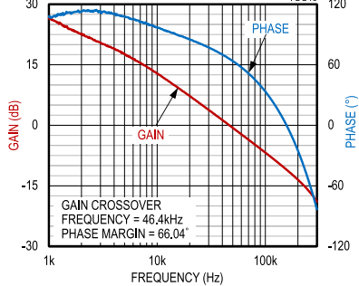
MAX17579/MAX17580, -5V OUTPUT, BODE PLOT, FIGURE 5 CIRCUIT
