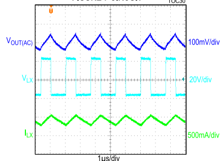
MAX17579/MAX17580, -15V OUTPUT, STEADY-STATE, FIGURE 7 CIRCUIT
