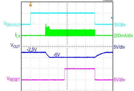
MAX17580, -5V OUTPUT, SOFT-START AND SHUTDOWN WITH PREBIAS VOLTAGE OF -2.5V, FIGURE 5 CIRCUIT
