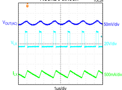
MAX17579, -5V OUTPUT, STEADY-STATE, FIGURE 5 CIRCUIT
