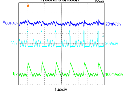
MAX17580, -5V OUTPUT, STEADY-STATE, FIGURE 5 CIRCUIT
