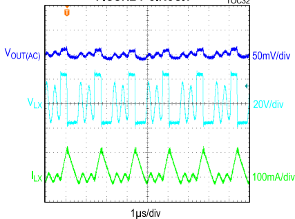
MAX17580, -15V OUTPUT, STEADY-STATE, FIGURE 7 CIRCUIT
