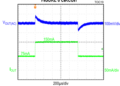
MAX17579, -5V OUTPUT, LOAD TRANSIENT BETWEEN 75mA AND 150mA, FIGURE 6 CIRCUIT
