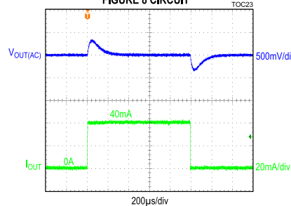
MAX17579, -15V OUTPUT, LOAD TRANSIENT BETWEEN 0A AND 40mA, FIGURE 8 CIRCUIT
