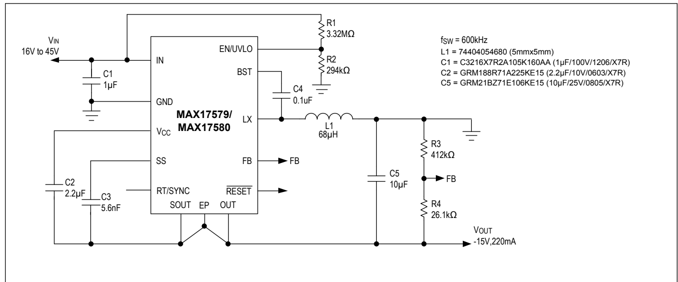
Figure 7. MAX17579 and MAX17580 -15V Output Application Circuit Compatible with 24V Input Bus Voltage
