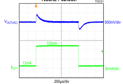
MAX17580, -15V OUTPUT, LOAD TRANSIENT BETWEEN 12mA AND 120mA, FIGURE 7 CIRCUIT
