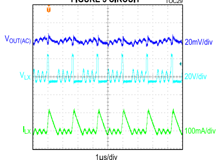
MAX17580, -5V OUTPUT, STEADY-STATE, FIGURE 5 CIRCUIT
