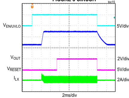
SOFT-START WITH PREBIAS VOLTAGE OF 2.5V FIGURE 3 CIRCUIT
