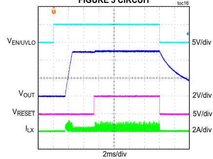
SOFT-START/SHUTDOWN FROM EN/UVLO FIGURE 3 CIRCUIT
