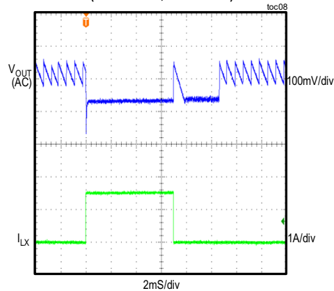
LOAD CURRENT STEPPED FROM 5mA TO 1.5A (5V OUTPUT, PFM MODE) toc08
