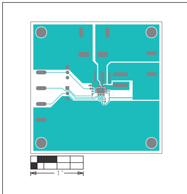
MAX17574 5V EV Kit—Top
