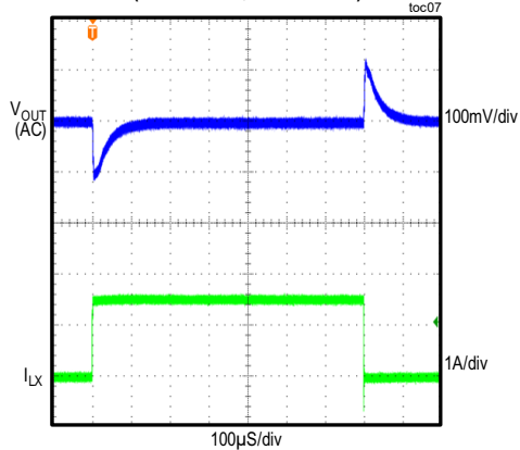
LOAD CURRENT STEPPED FROM NO LOAD TO 1.5A (5V OUTPUT, PWM MODE) toc07
