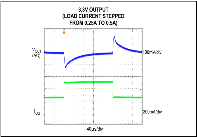
Figure 4. MAX17541G 3.3V Output 250mA to 500mA Load Transient
