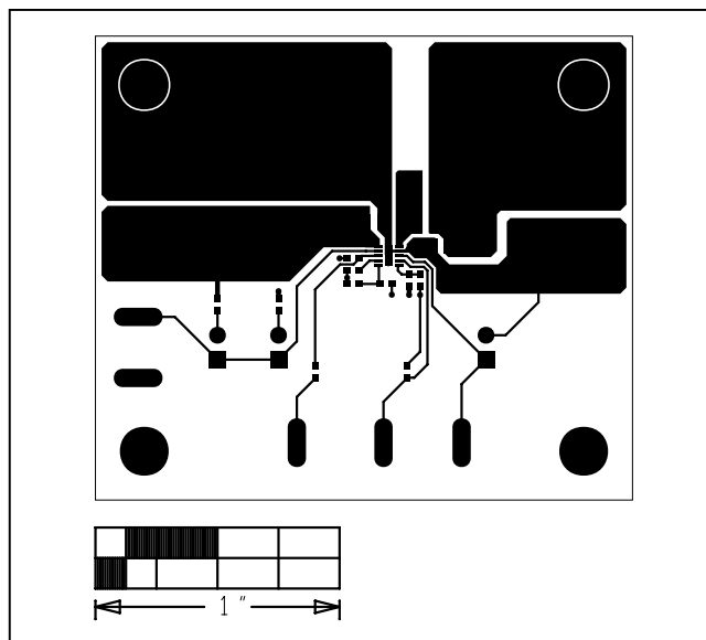
Figure 2. MAX17530 5V EV Kit (TDFN) PCB Layout—Component Side
