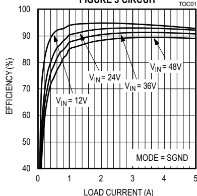
EFFICIENCY vs. LOAD CURRENT 5V OUTPUT, PWM MODE, FIGURE 3 CIRCUIT
