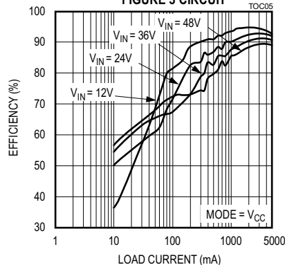
EFFICIENCY vs. LOAD CURRENT 5V OUTPUT, DCM MODE, FIGURE 3 CIRCUIT
