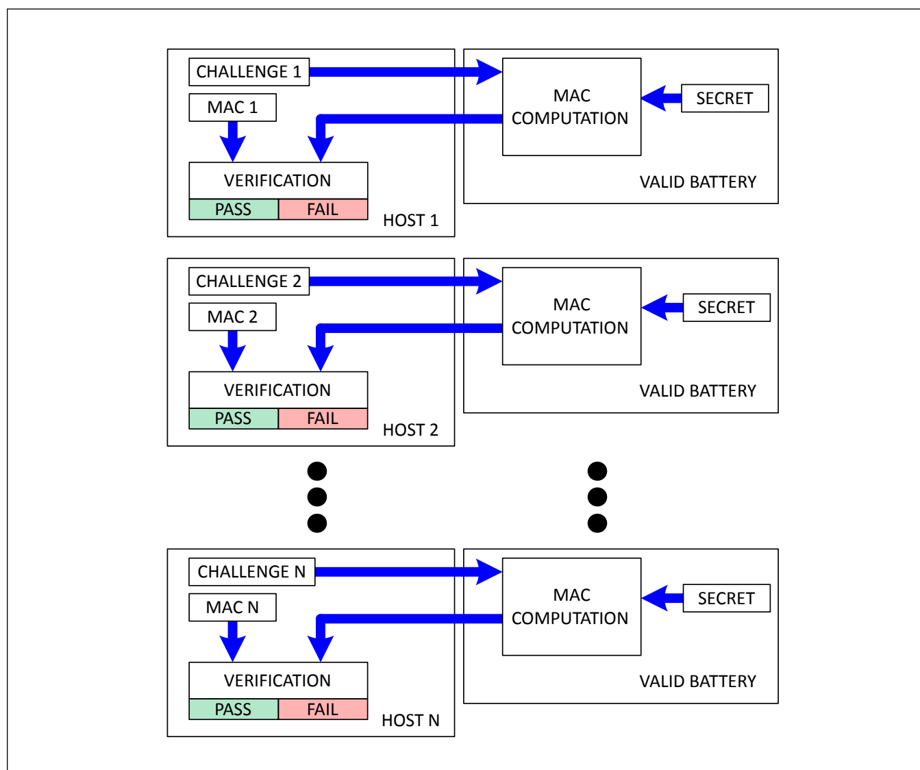
Figure 31. Battery Authentication without a Host Side Secret
