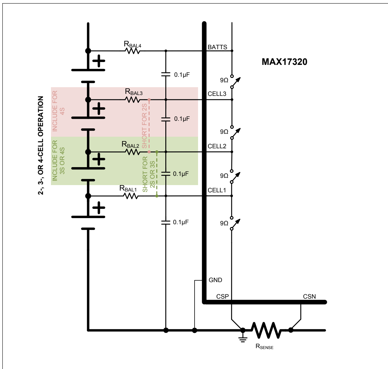
Figure 23. Cell Balancing Configuration
