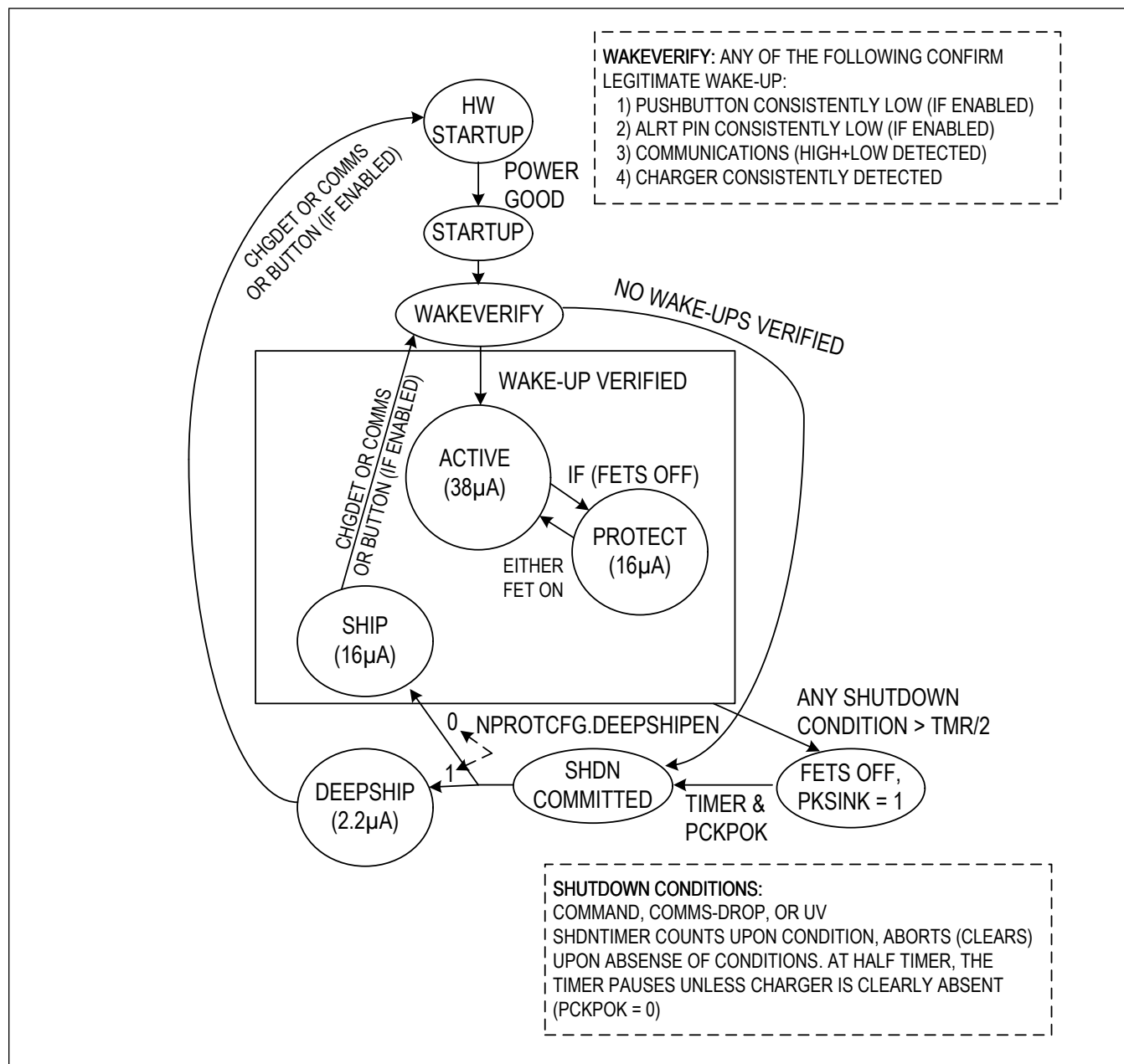
Figure 25. Power Modes Transition State Diagram
