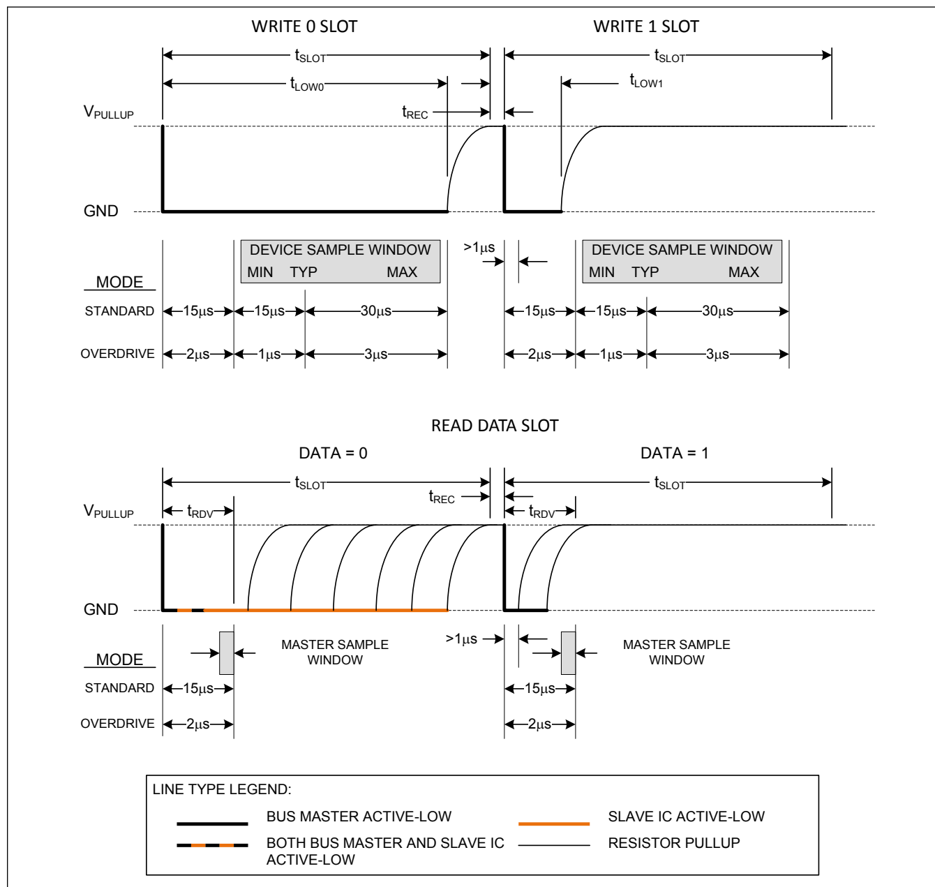
Figure 46. 1-Wire Write and Read Time Slots
