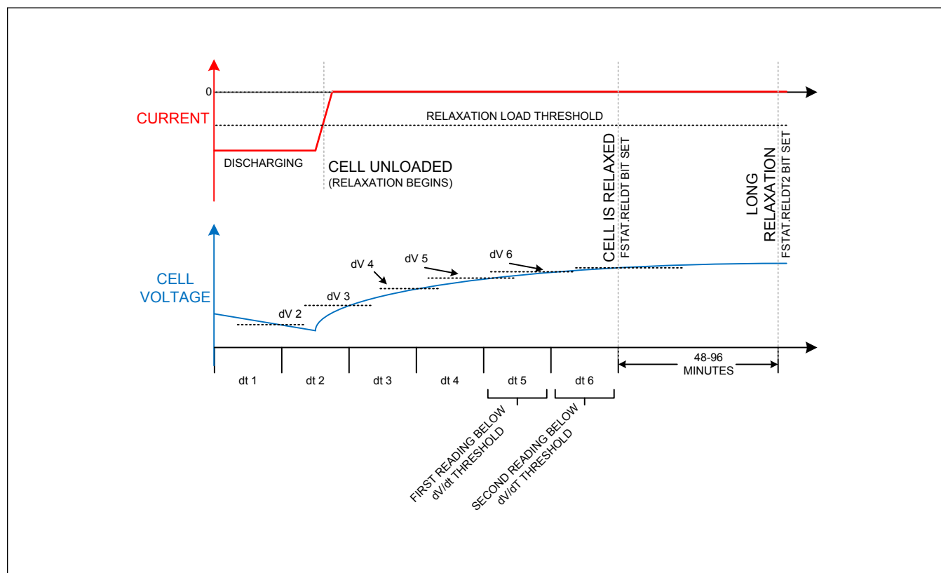
Figure 27. Cell Relaxation Detection
