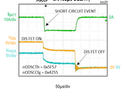
SHORT-CIRCUIT PROTECTION ( I_{SCCP} = 5\text{A}/192\mu\text{s DELAY} )
