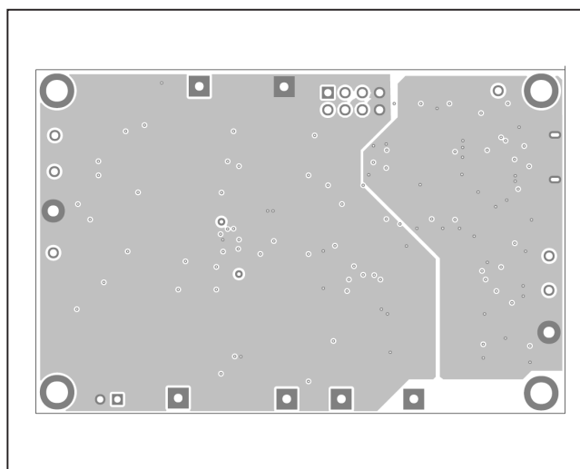
MAX173x0G EV Kit Layout—Layer 2
