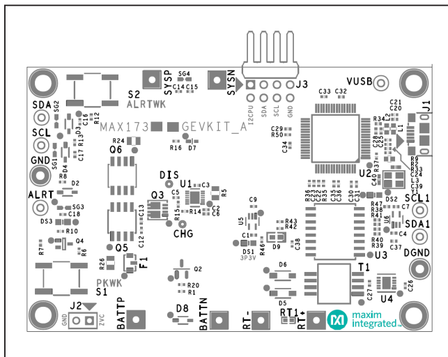
MAX173x0G EV Kit Component Placement Guide—Top Silkscreen
