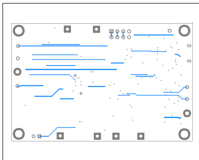
MAX173x0G EV Kit Layout—Bottom Layer
