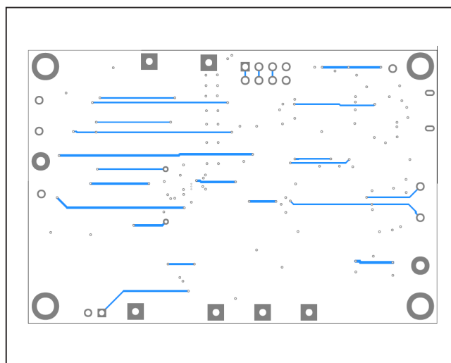
MAX173x0X EV Kit Layout—Bottom Layer
