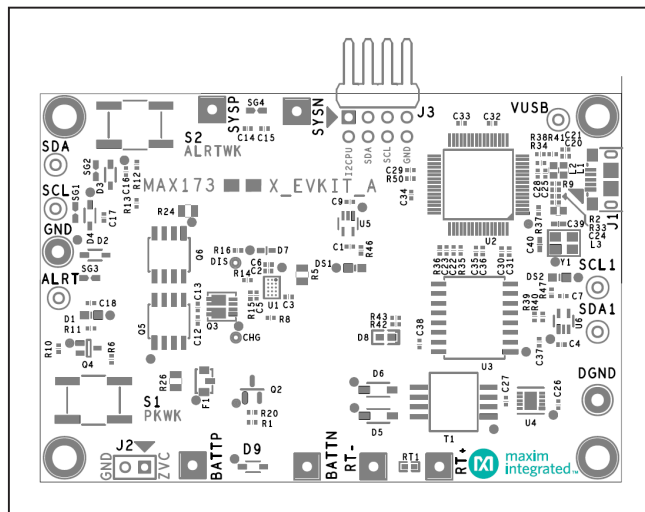
MAX173x0X EV Kit Component Placement Guide—Top Silkscreen
