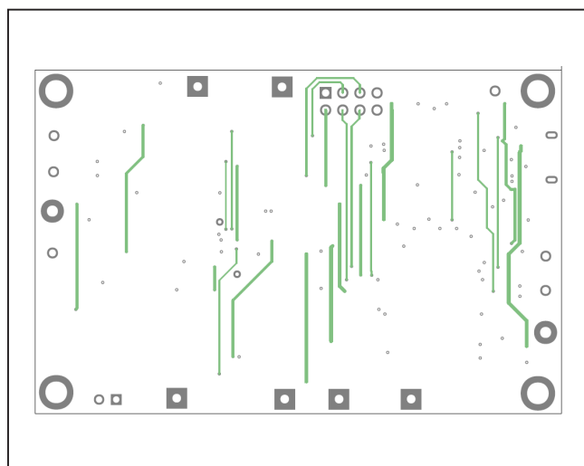
MAX17300G EV Kit Layout—Layer 3
