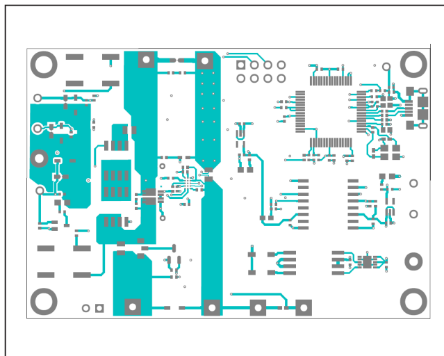
MAX173x0X EV Kit Layout—Top Layer
