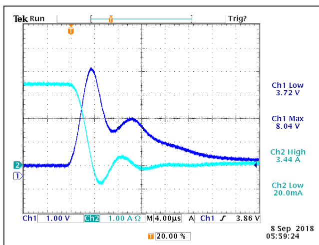
Figure 23. BATT Voltage and Battery Current Waveform at Overcurrent Protection Event with Bad Connections
