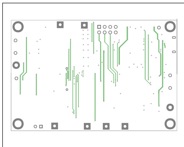
MAX173x0X EV Kit Layout—Layer 3
