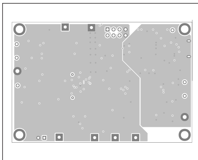
MAX173x0X EV Kit Layout—Layer 2
