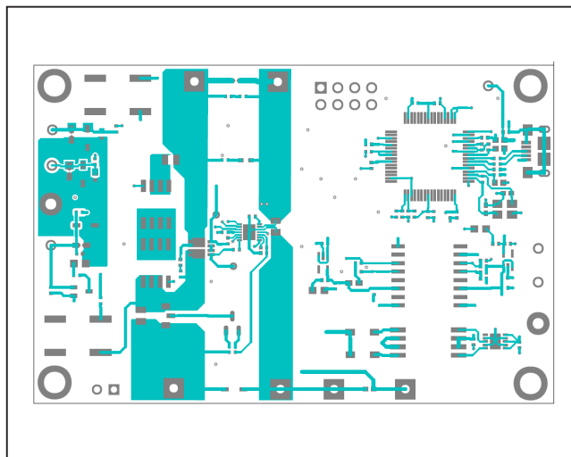
MAX173x0G EV Kit Layout—Top Layer
