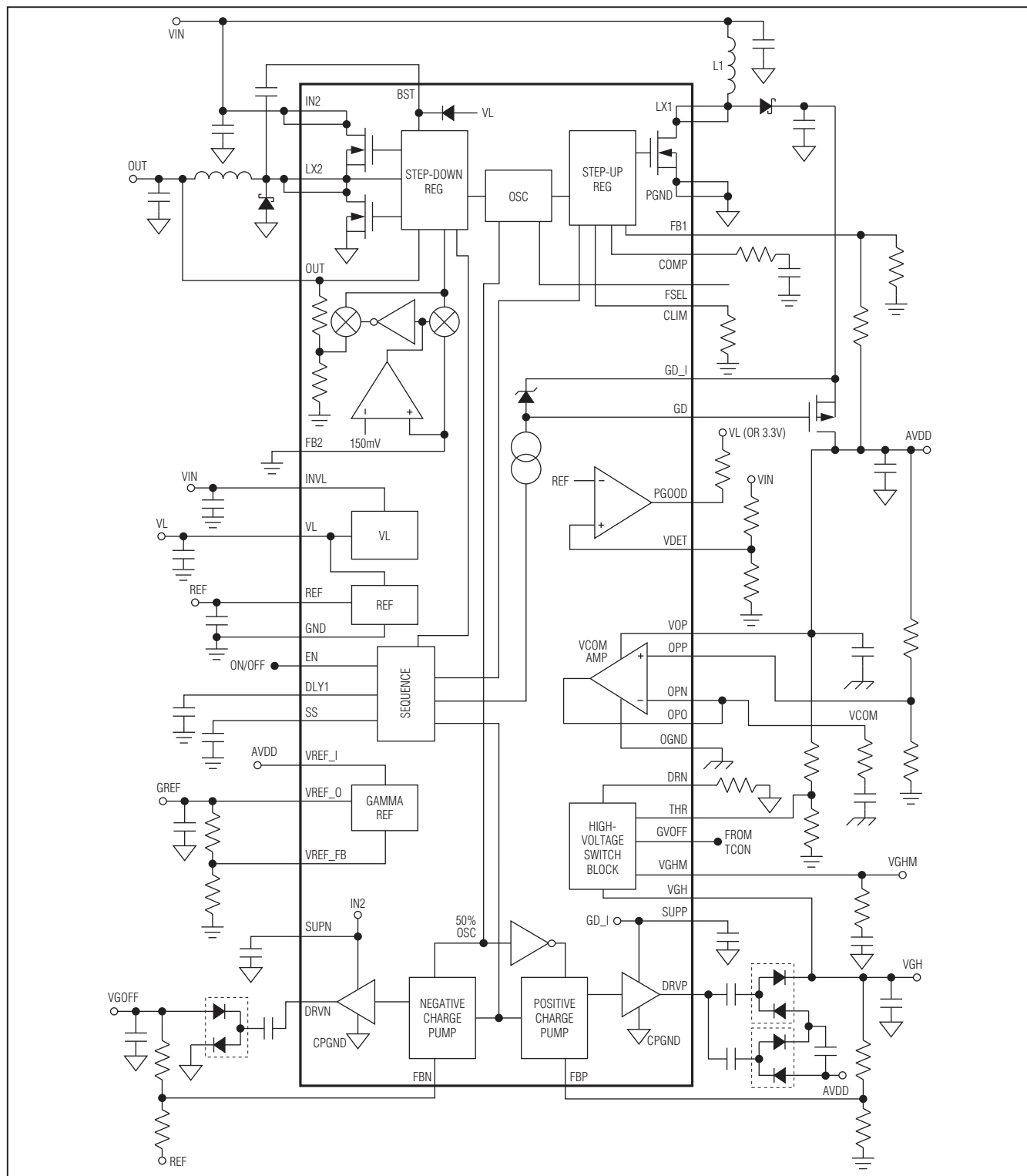
Figure 2. Functional Diagram
