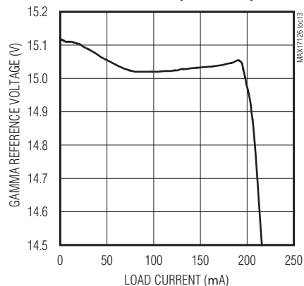
GAMMA REFERENCE LOAD REGULATION ( V_{REF} = 16\text{V} )
