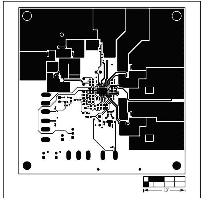
Figure 3. MAX17085B EV Kit PCB Layout—Component Side
