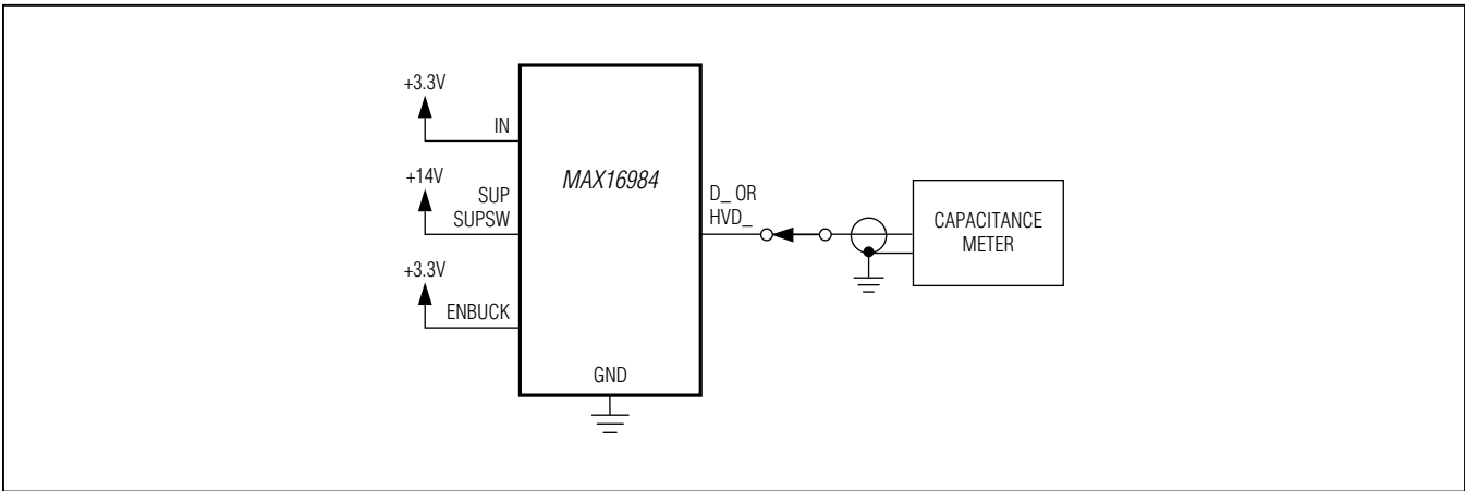
Figure 4. On-Capacitance
