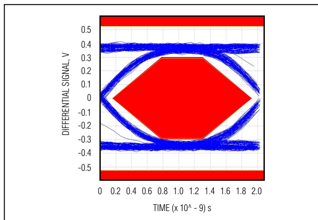
Figure 16. Tuned Far Eye Diagram, 3-Meter Cable
