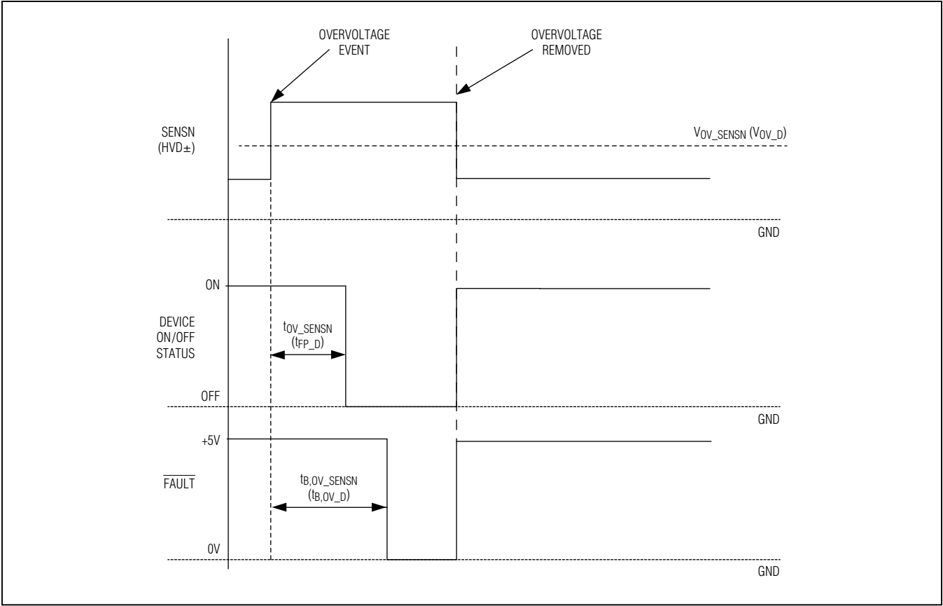
Figure 1. Overvoltage Detection on SENSEN, HVD+, HVD- Timing Diagram
