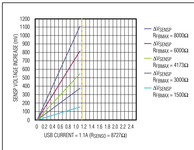
Figure 10. Increase in SENSE vs. USB Current
