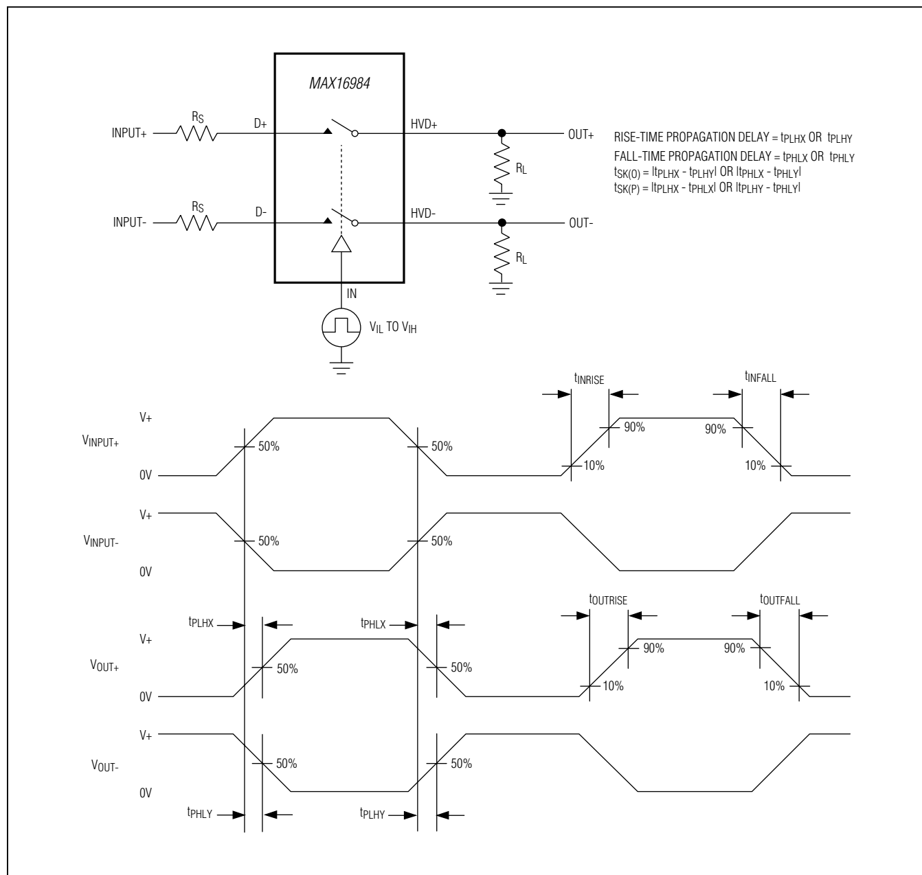
Figure 5. Propagation Delay and Output Skew
