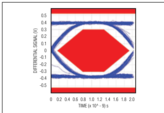
Figure 14. Tuned Near Eye Diagram (with Data Switch)
