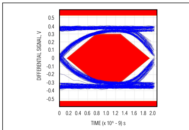
Figure 15. Untuned Far Eye Diagram, 3-Meter Cable
