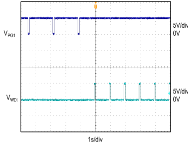
WATCHDOG DE-ASSERTION
