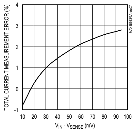
TOTAL CURRENT MEASUREMENT ERROR vs. (V IN - V SENSE )
