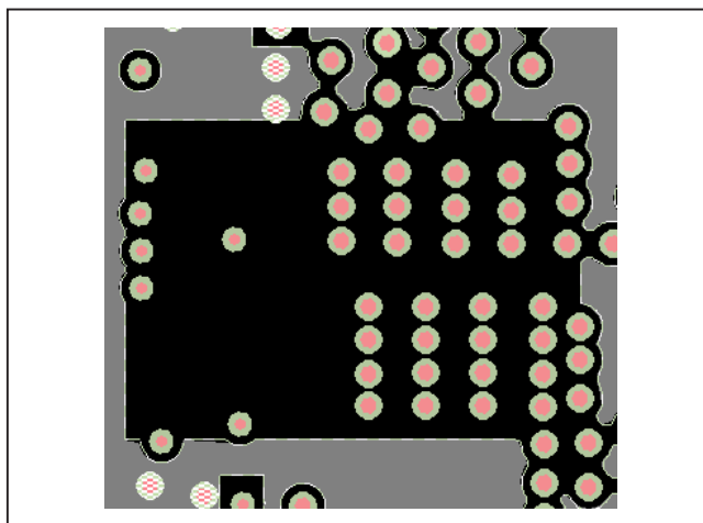
Figure 9. Second Layer (GND) with Keepout
