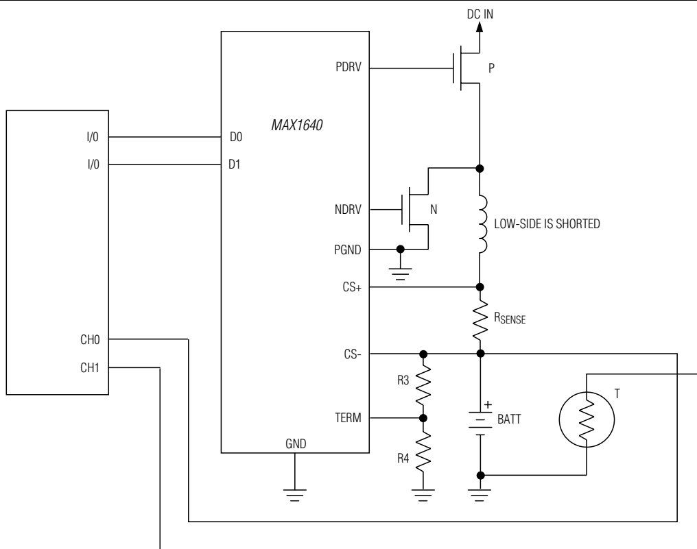
Figure 4. Microcontroller Battery Charger
