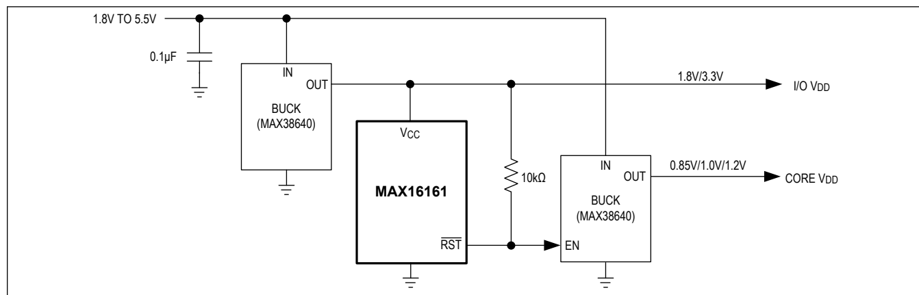
Figure 8. MAX16161 as a Simple Power Supply Sequencer
