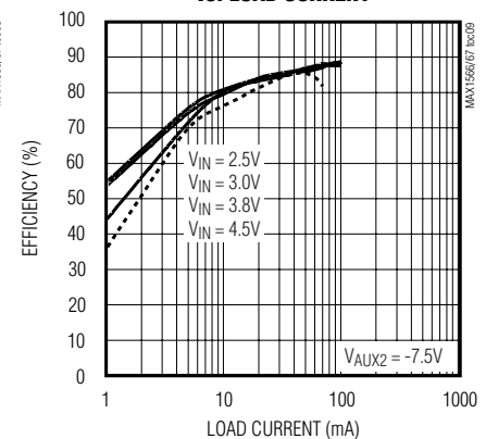
MAX1567 AUX2 EFFICIENCY vs. LOAD CURRENT
