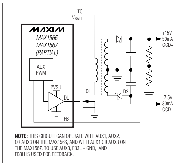
Figure 9. \pm 15V and -7.5V CCD Bias with Transformer
