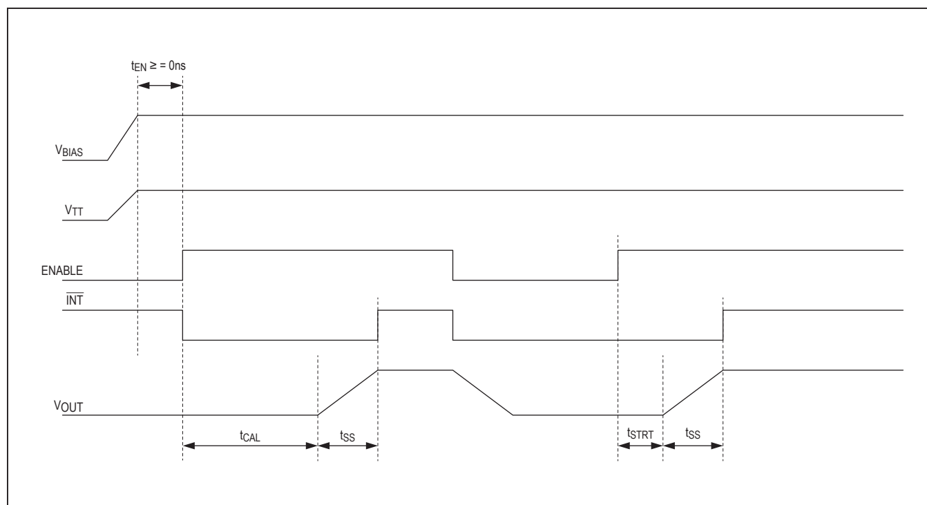
Figure 7. Startup Sequence
