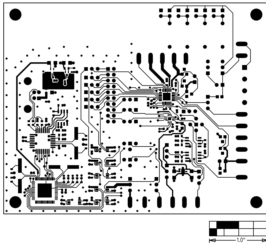
Figure 4. MAX15501 EV Kit PCB Layout—Component Side
