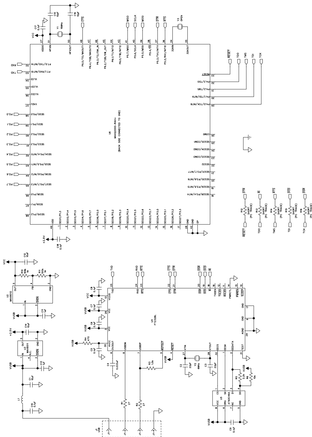
Figure 2b. MAX15501 EV Kit Schematic (Sheet 2 of 2)
