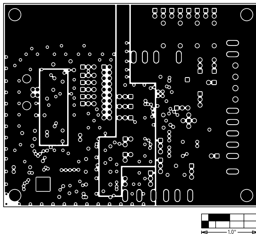
Figure 6. MAX15501 EV Kit PCB Layout—Layer 3
