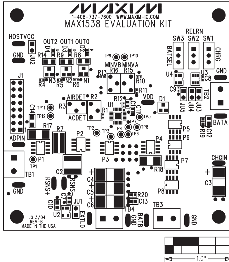
Figure 3. MAX1538 EV Kit Component Placement Guide—Component Side
