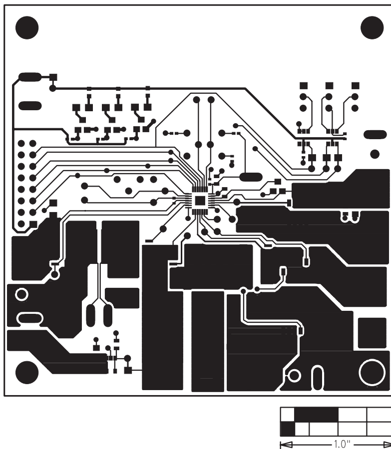
Figure 4. MAX1538 EV Kit PC Board Layout—Component Side
