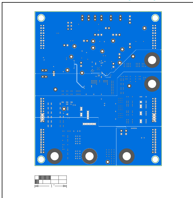
MAX15157D EV Kit PCB Layout—Layer 4
