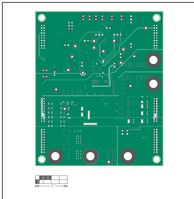
MAX15157D EV Kit PCB Layout—Layer 3
