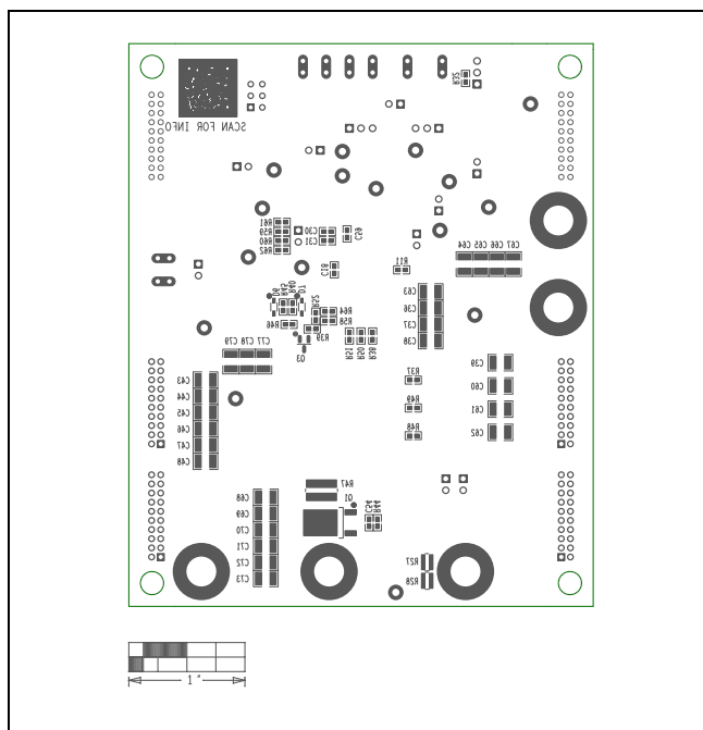
MAX15157D EV Kit Component Placement Guide—Bottom Silkscreen
