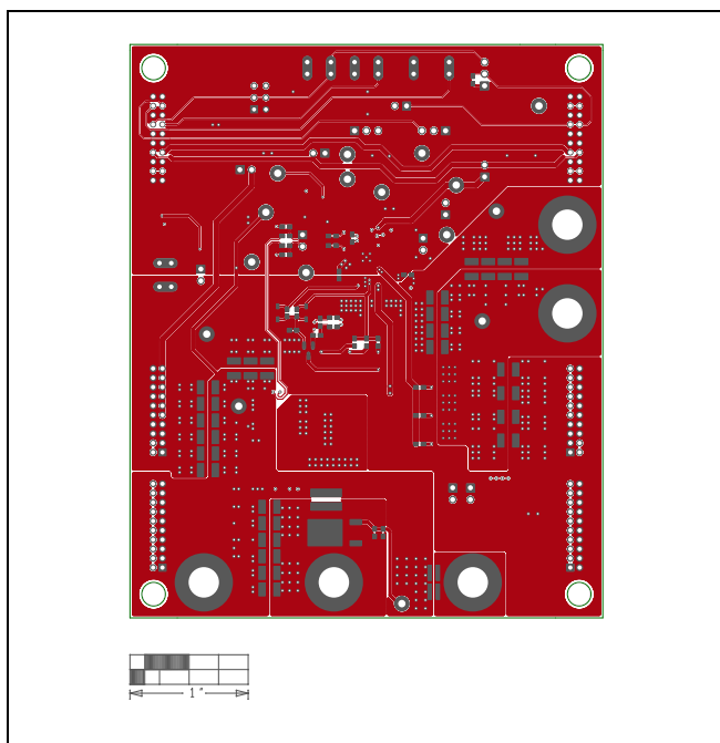
MAX15157D EV Kit PCB Layout—Bottom
