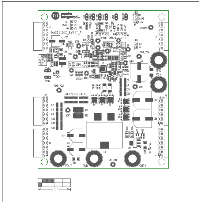
MAX15157D EV Kit Component Placement Guide—Top Silkscreen
