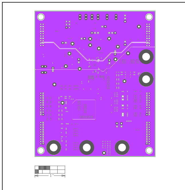
MAX15157D EV Kit PCB Layout—Layer 5
