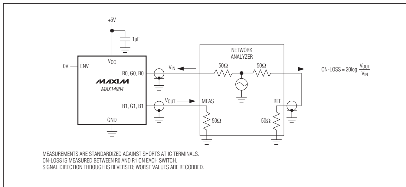
Figure 2. On-Loss
