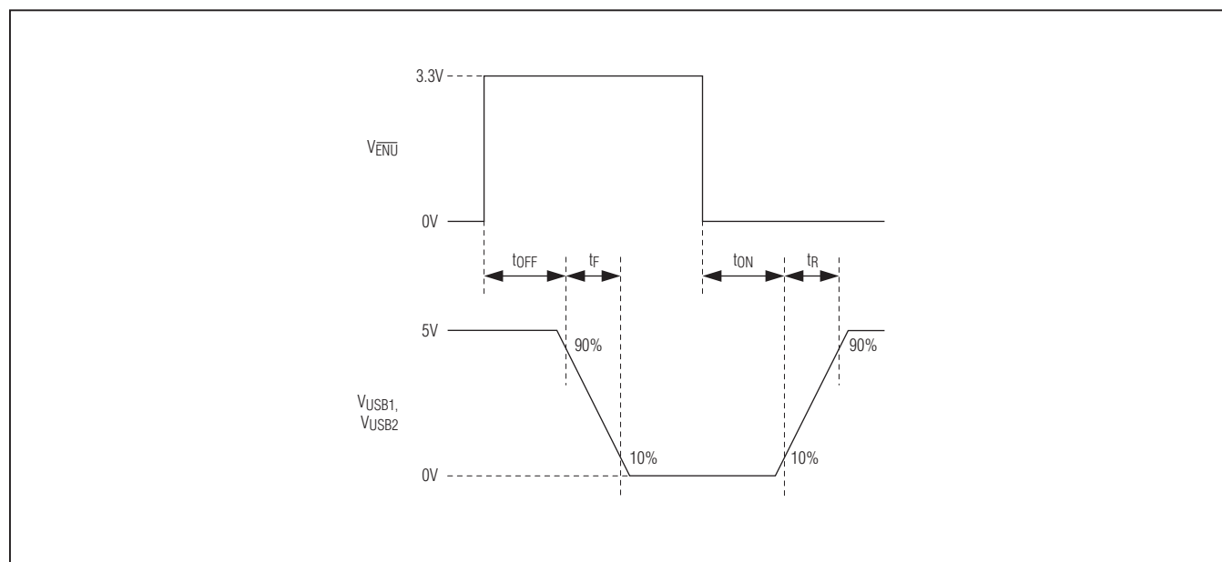
Figure 1. Timing Diagram for USB Switch Parameters
