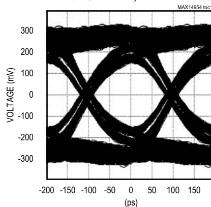
INEQ0 = INEQ1 = 0, VIN = 200mVp-p, 0EQ2 = 1, 0EQ1 = 0, 0EQ0 = 1, OUTPUT AFTER 19in STRIPLINE, DATA RATE = 5GT/s
